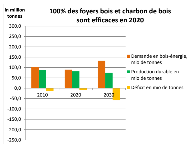
Figure 23: Foyers améliorés efficaces en 2020
