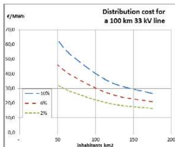
Figure 17: Optimised rural distribution cost for a 33 kV line
